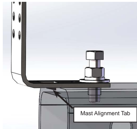
Diagram 10N. Mast alignment
