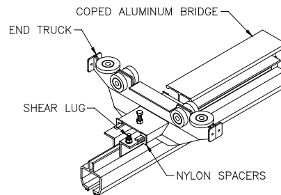
Diagram 5C. Installing clamping end truck on coped aluminum bridge. See NOTE .
