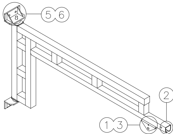
WSJ200 Wall/Column Mounted Crane
