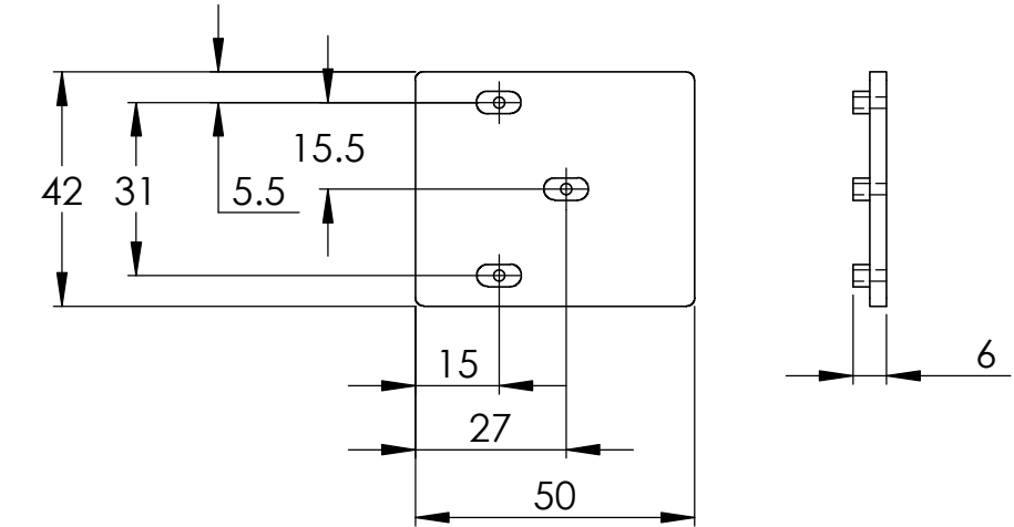
MOUNTING PLATE DETAIL
