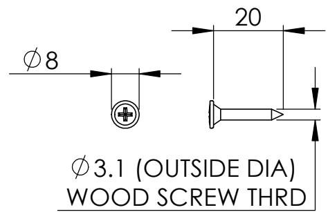
MOUNTING SCREW DETAIL
